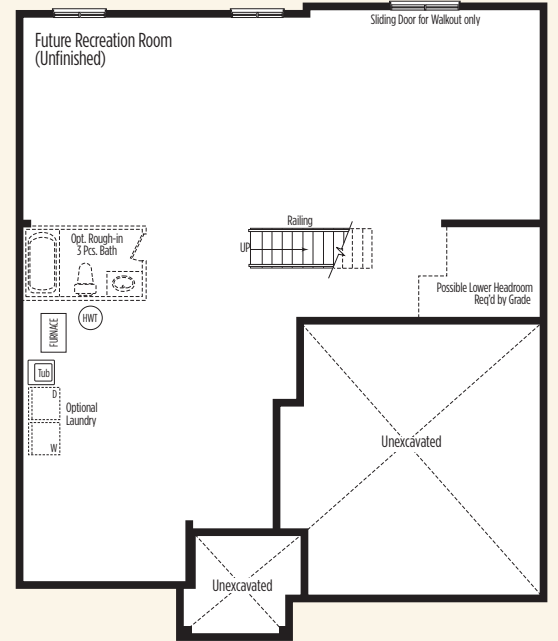
UNFINISHED BASEMENT PLAN
